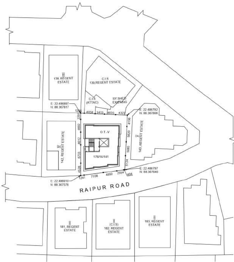
SITE PLAN
